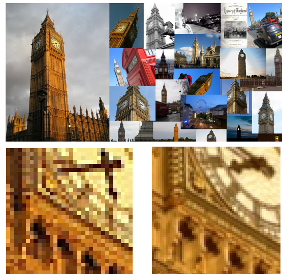
Figure 10: Online Database: Our algorithm can derive relationships between photographs in image databases like Flickr. These relations enable us to add specific details. Top: A subset of the first 35 images for the query Big Ben on Flickr. The enlarged image on the left was then chosen by the user. Bottom left: Detail of the original image. Bottom right: Result by our algorithm. A closeup on the small turret in the bottom right of the root image is given in Figure 11.
