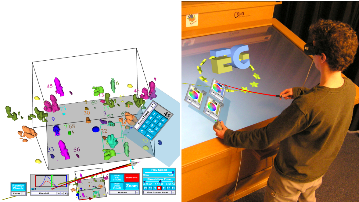
Figure 16: Hybrid Interfaces: The new Cloud Explorer interface consists of multiple organized 3D windows and widgets (left). The interaction support allows the use of smaller interface elements. The small color picking widgets on the tracked PlexiPad are still usable despite tracking inaccuracies and hand jitter (right).
