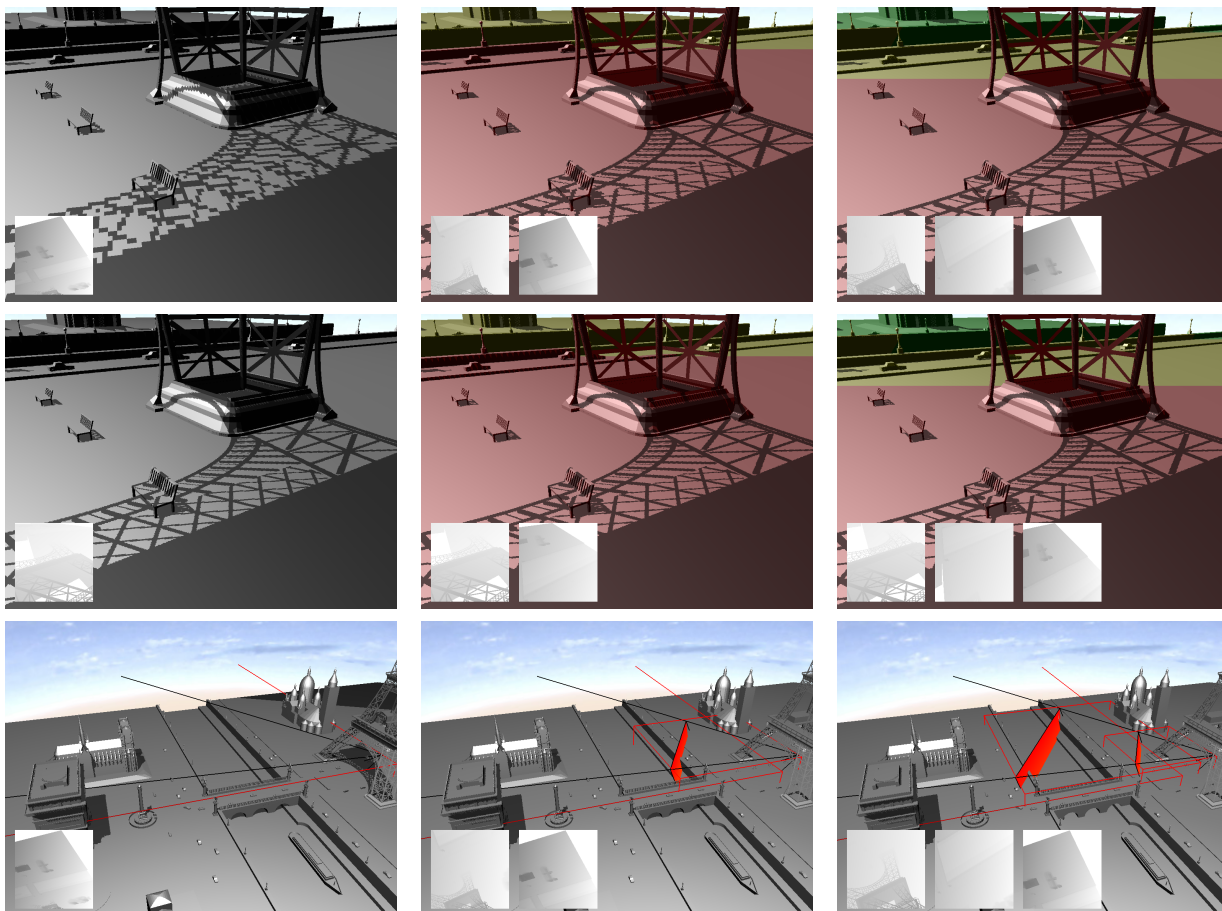
Figure 3.3 Examples of global partitioning along the z -direction with and without warping for one to three partitions (left to right). The shadow map used for each fragment is color coded: camera view, uniform (top row); camera view, with reparametrization (middle row); and outside view showing the view frustum, the partitions, and the intersection bodies (bottom row). Inlays show the depth maps.
