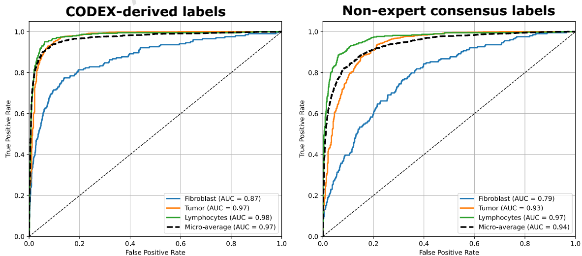
Figure 5. The receiver operator curves (ROC) with area under the curve (AUC) metrics of the trained models on the test set.
