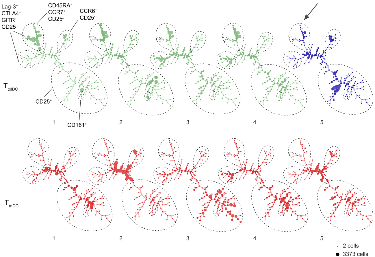
Fig. 3. Multidimensional SPADE analysis of T_{tolDC} and T_{mDC} lines. T_{tolDC} lines (green) show differential cluster distribution in the SPADE analysis from the T_{mDC} lines (red). The non-suppressive T_{tolDC} line (blue) shows different distribution than the suppressive T_{tolDC} lines. Circles depict clusters with designated marker expression as shown in Supplementary Fig. 1 . The grey arrow indicates the clusters lacking in the non-suppressive T_{tolDC} line. (For interpretation of the references to colour in this figure legend, the reader is referred to the Web version of this article.)
