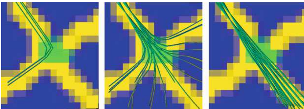
Fig. 7 Rotated 90° crossing. From left to right: streamline tractography for DTI, geodesic ray tracing for DTI, HARDI multi-valued geodesic
