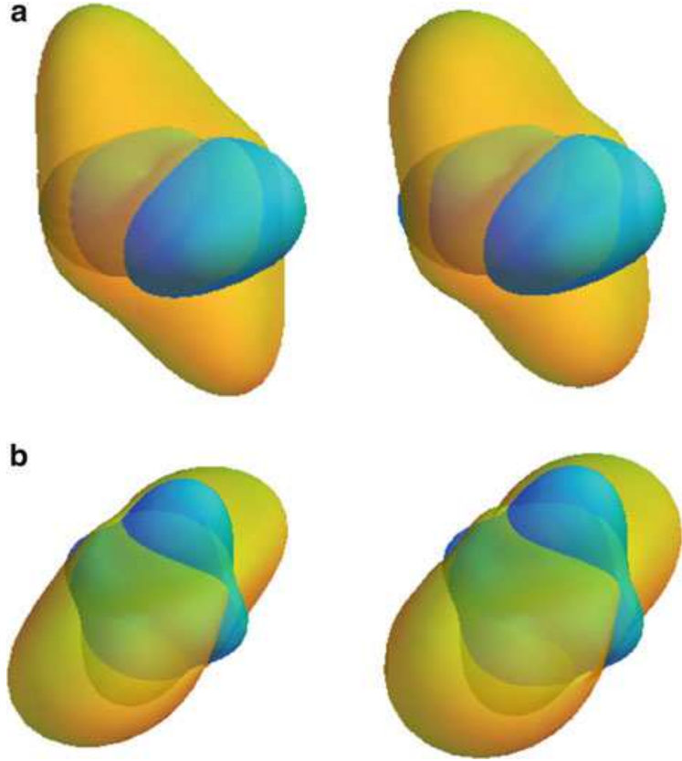
Fig. 3 ODF ( Blue ) and its inverse ( Yellow ) using least-squares fit ( Left ) and analytic inversion ( Right ). (a) ODF and its inverse for a single fiber profile. (b) ODF and its inverse for a crossing fiber profile
