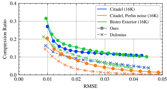
Figure 5: A plot showing compression ratio as a function of Root Mean Square Error (RMSE). Comparing our lossy method to Dolonius [DSKA17].
