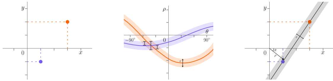
Figure 4: Two points in (x,y) space (left) and their representation in (\theta,\rho) space after Hough transform. (center). The intersection of the two lines in (\theta,\rho) space defines a line in (x,y) which passes through both points (right). To allow for approximate fitting we define an error margin e in \rho which corresponds to an euclidean error in (x,y) space. To accelerate the search we discretize \theta keeping only the overlapping values. The \rho bounds are stored in a continuous representation (center)
