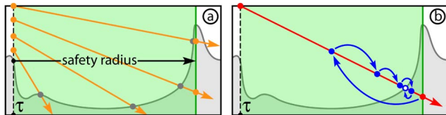
Fig. 3. Safety distance. (a) Every ray originating above the texel \tau intersects the surface at most once within the safety cylinder. (b) In this example, one marching step using the safety radius is enough to cross the surface: the bisection (blue) then finds the (unique) intersection.
