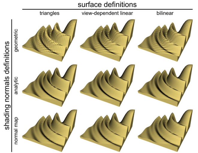
Fig. 25. Possible reconstructions for a 25^2 height field.
