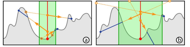
Fig. 18. Advantage of visibility restriction. (a) The safety distance defined for any ray is smaller than (b) the one for exterior rays only.
