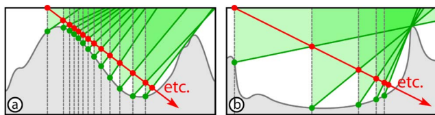
Fig. 2. Limitations of cones. (a) Marching silhouette rays is slow. (b) Concave zones cannot be reached in a finite number of steps (for clarity, only half-cones are drawn).
