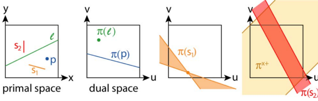
Fig. 19. Dual parametrization of 2D lines.
