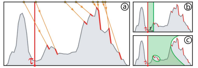
Fig. 23. Safety shapes from limiting triangles. (a) Limiting triangles (red) for texel \tau and associated limit rays (orange). (b) Safety distance (cylinder). (c) General safety shape empty of limiting triangles.
