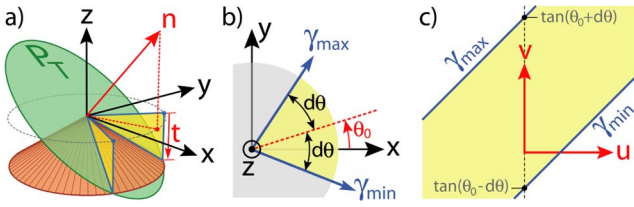
Fig. 22. Viewing angle restriction. (a) Intersection of \mathcal{P}_T (with normal n ) with a cone of slope t = \tan \phi_{\max} defines a restricted angular sector. (b) 2D projection of this angular sector: \theta_0 is the direction of the projection of n . (c) This corresponds to two half-planes in dual space.
