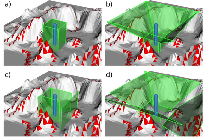
Fig. 28. The four variants of safety shapes. (a) Isotropic safety distance. (b) Isotropic cylinder-cone. (c) Directional SD. (d) Directional CC.
