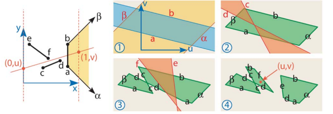
Fig. 21. Accurate rayset computation in the dual parametrization. (1) Initialization with rays hitting [ab] , directed between \alpha = (1, -1) and \beta = (1, 1) : R_0 \leftarrow \pi([ab]) \cap \pi^{x+} = (a, \alpha, b, \beta) . (2) Removal of rays blocked by [cd] : R_1 \leftarrow R_0 \setminus \pi([cd]) = ((a, c, d, \beta), (a, \alpha, b, c, d)) . (3) Further with [ef] : R_2 \leftarrow R_1 \setminus \pi([ef]) = ((a, c, d, \beta), (d, f, b, c), (a, \alpha, b, e, d)) . (4) A point (red) in the residual dual area discloses a ray from \mathbb{R}^{x+} hitting [ab] without hitting [cd] and [ef] .
