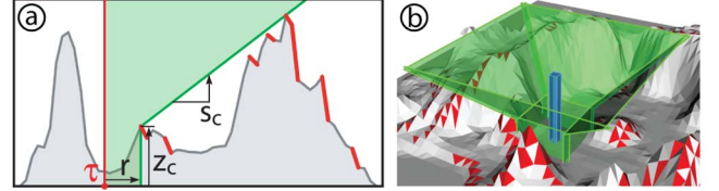
Fig. 24. Hybrid cylinder-cone safety shape. (a) The three parameters. (b) Example in 3D.
