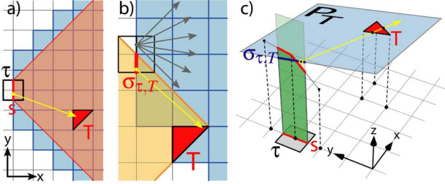
Fig. 17. Limiting triangles. (a) The \pm 45^\circ quadrant leaving from s_\tau defines possible locations of limiting triangles. (b) Definition of \sigma_{\tau,T} in a case where it does not entirely cover s_\tau . (c) Here, a point of \sigma_{\tau,T} above S exists, thus T is limiting (a limit ray leaves this point).
