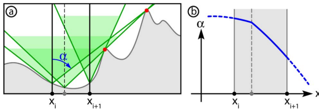
Fig. 10. Interpolation of cones inside a texel. (a) Cones are bound by pivot points, changing arbitrarily when the cone position moves between two neighboring samples. (b) This results in a discontinuous derivative for the cone's angle.
