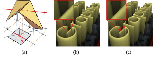
Fig. 27. Handling of null safety distances. (a) A zero safety distance is affected to the shown texel, requiring at most two simple iterations to escape from it without missing intersections; rendering (b) without and (c) with clamping of safety distances to value one (notice the small artifacts on sharp edges in the latter case).
