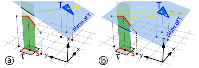
Fig. 15. Limiting triangle. (a) A ray hitting the back face of T is found, making it a limiting triangle. (b) T is not limiting as any ray leaving above h(s) sees his front face.
