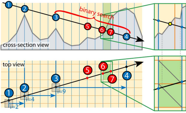
Fig. 14. The improved algorithm: the three first steps fetch a value i from the precomputed safety distances map to jump on x -centerlines, the fourth step falls below the surface, which switches to the bisection phase.
