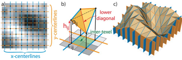
Fig. 12. Surface definition from a sampled height map. (a) Height-map samples and centerlines. (b) Triangulation for an intertexel. (c) Complete surface.
