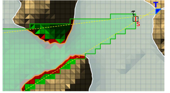
Fig. 20. Potential blockers (orange) for rays going from s to T are found in the shaft-like shape (green).
