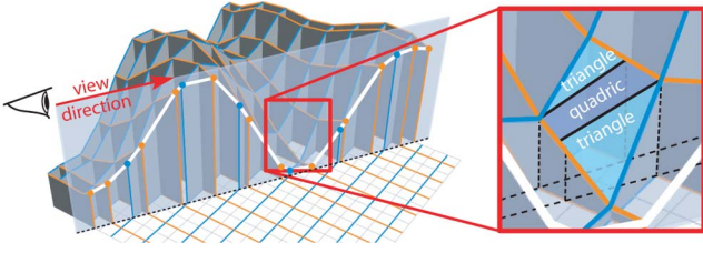
Fig. 26. View-dependent linear approximation of the height map along the viewing direction: in each texel, this corresponds to a continuous view-dependent surface, made of two triangles and one quadric patch.
