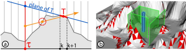
Fig. 16. Limiting triangles bound the safety distance. (a) A ray hitting the back face of a limiting triangle necessarily crosses the surface earlier, so that the safety distance is less than or equal to k . (b) Safety planes for each of the four ray classes (limiting triangles are shown in red).
