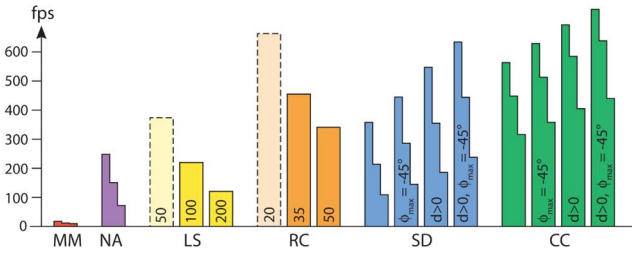
Fig. 29. Timings: MM [23], NA (our naive solution), LS [21], RC [30], SD (our safety distance), CC (our cylinder-cone). For LS and RC, numbers denote marching iterations. For SD and CC, \phi_{max} is taken as 90^\circ if not specified (i.e., no viewing angle restriction); d > 0 corresponds to the strictly positive distance assumption (Section 7). Dashed boxes denote situations where rendering artifacts are too strong to allow usefulness. For each bar, the three stair levels correspond to height-field resolutions 256^2 , 512^2 , and 1,024^2 .
