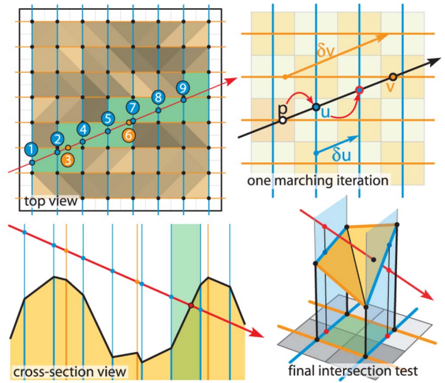
Fig. 13. Successive steps of the naive marching algorithm.
