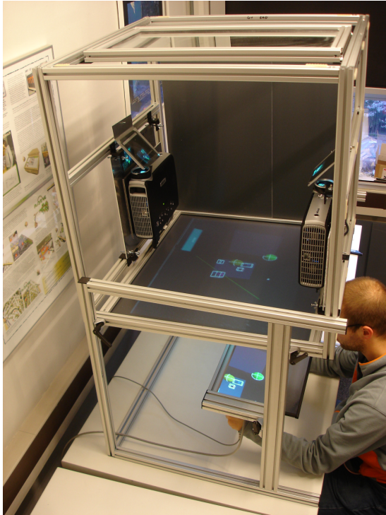
Figure 2: The inside of the PDRIVE. Two projectors in a mirrored configuration project against an overhead mirror. The image is reflected down onto the screen, which the user views by looking into a second mirror, or user mirror. The user's hands go behind the second mirror, offering co-location between the user's hands and the virtual objects.
