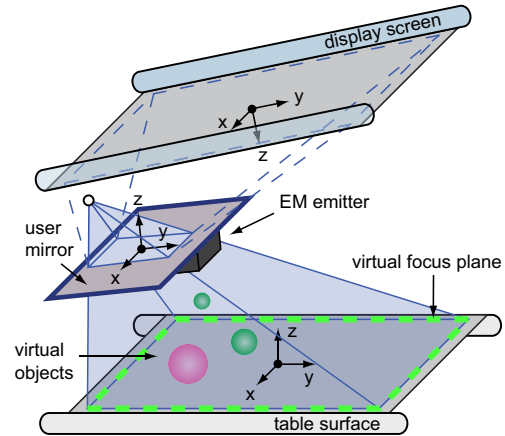
Figure 6: Coordinate frames used for tracking and tracking setup. The electromagnetic emitter is mounted under the user mirror. During a calibration process, the relation between the coordinate frames for the screen, mirror and table are derived. The relation between the mirror and screen determines the virtual focus plane.
