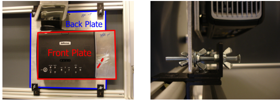
Figure 5: Left: The projector mount, which consists of two aluminum plates. The projector is fixed to the front plate, which is then fixed to the back plate so that the front plate can be rotated. Right: The brackets used to fix the projector mounts to the frame. These allow each corner of the projector mounts to be transversally translated.
