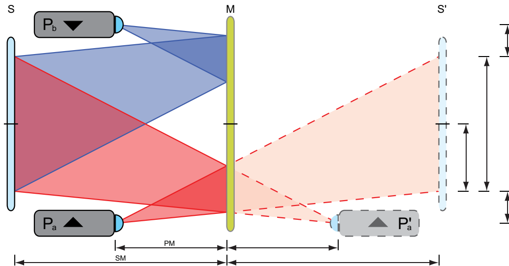
Figure 4: Layout of optical components to obtain an optimal, factory tuned rectangular image with two projectors. We take advantage of horizontal symmetry of off-the-shelf projector optics, and therefore can flip the second projector. The angle between projector and screen needs to be 90 degrees, and mirror needs to be parallel to the screen
