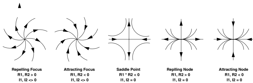
Fig. 2. Vector field topology: critical points are usually classified by the eigenvalues of the Jacobian [21]. R represents the real components and I the imaginary components of the Jacobian.
