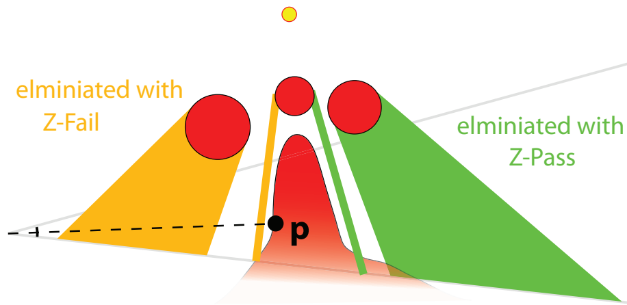
Figure 2.9 Split-Shadow Volume
