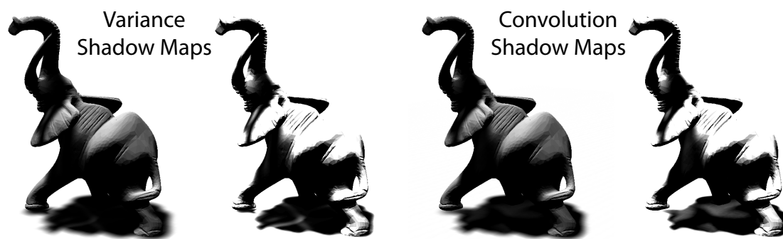
Figure 4.9 Although some light bleeding is present in approximate solutions (VSM: left, CSM: right, each original and scaled with a factor four), newer approaches show significantly less artifacts and are a good choice when high performance is needed.
