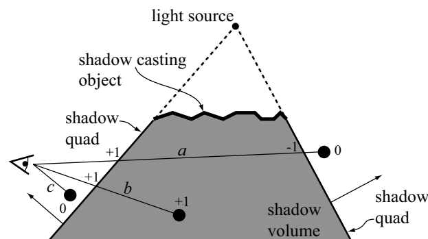
Figure 2.6 The standard shadow volume algorithm. Ray b is in shadow, since the stencil buffer has been incremented once, and the stencil buffer values thus is +1. Rays a and c are not in shadow, because their stencil buffer values are zero. (Courtesy of Tomas Akenine-Möller)
