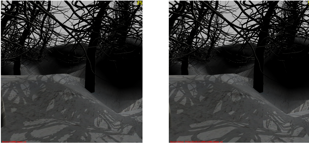
Figure 3.14 Left: standard 4096^2 shadow map. Right: QVSM with a maximum refinement level of 32 \times 32 , and 2048^2 tiles.
