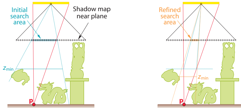
Figure 5.9 The intersection of the shadow map near plane with the point-light pyramid yields an initial search area for extracting occluder approximations. If the minimum depth z_{min} of this area is known, it becomes possible to refine the search area iteratively.
